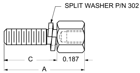
PREASSEMBLED LOCK WASHER
